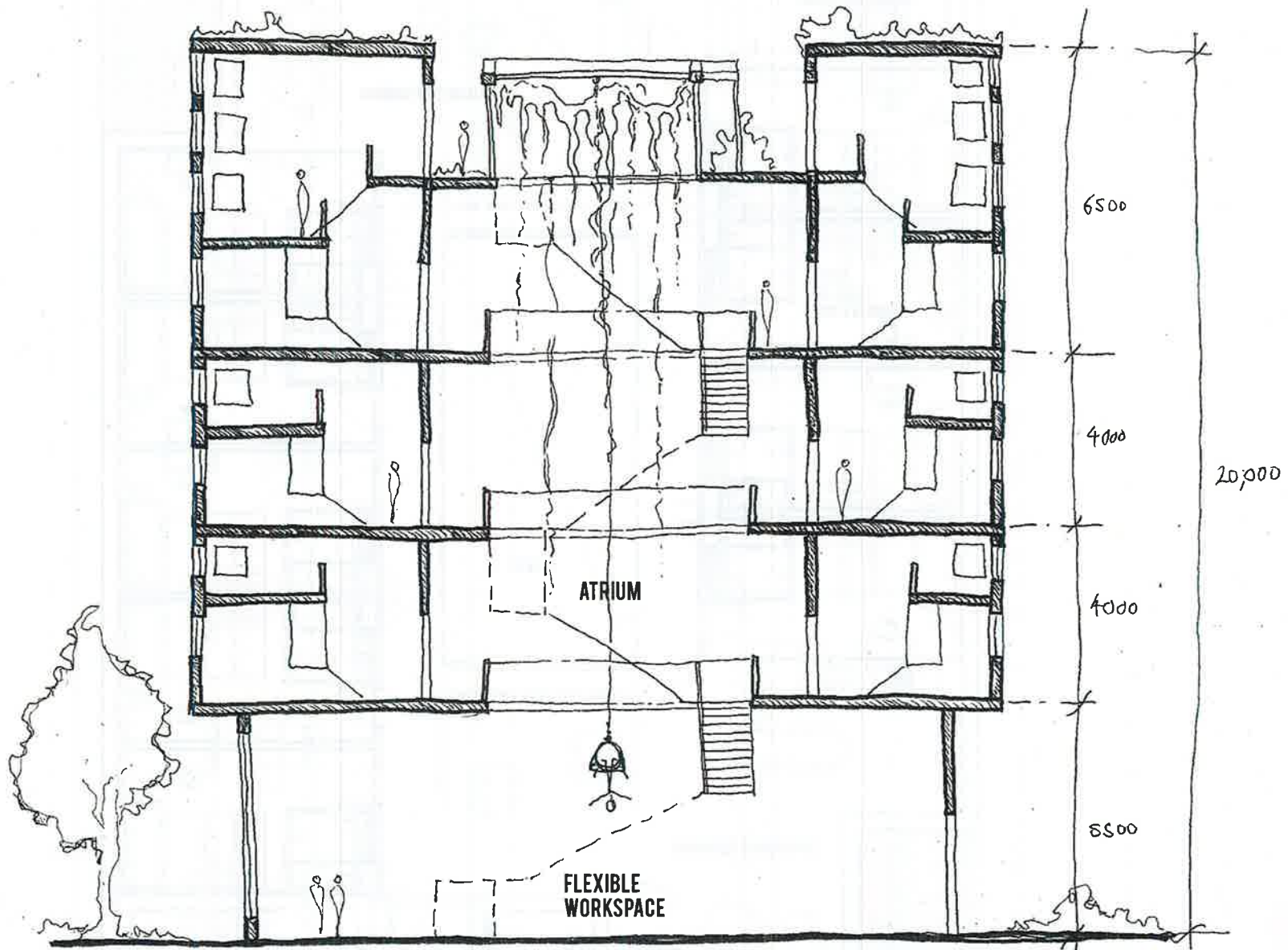
ILLUSTRATIVE SECTION
