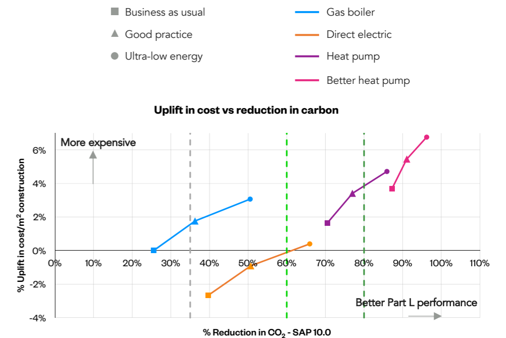
Figure 48 - Mid-rise apartment building - Additional construction costs vs Part L reduction based on system chosen
